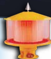
Medium Intensity 2,000 candela (Flashing Red OR Fixed Red LEDs)
